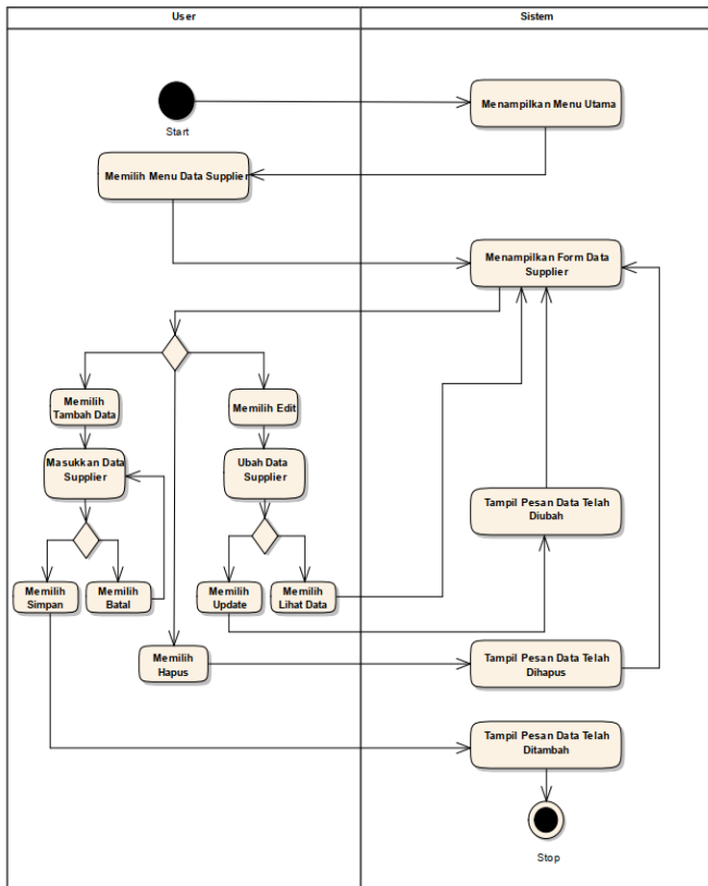
Gbr 3. Activity Diagram User Mengelola Data Supplier
