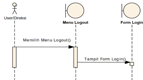
Gbr 19. Sequence Diagram Logout
