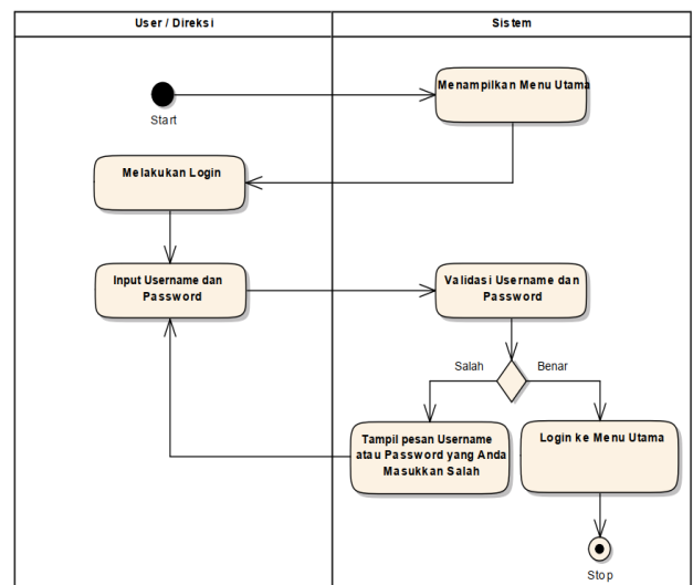
Gbr 2. Activity Diagram User/Direksi Melakukan Login
