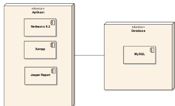
Gbr 20. Deployment Diagram
